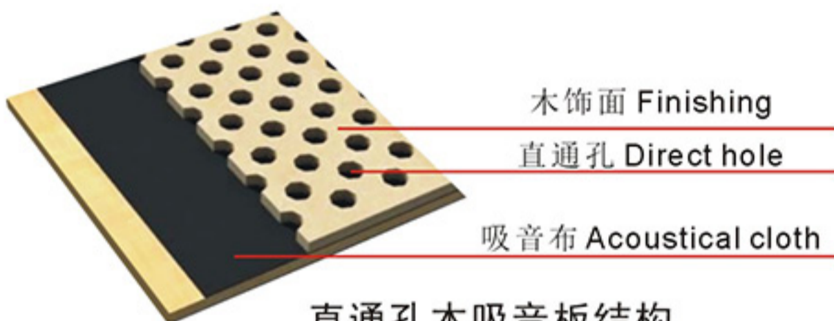
直通孔木吸音板结构 Direct hole acoustic panel instruction
